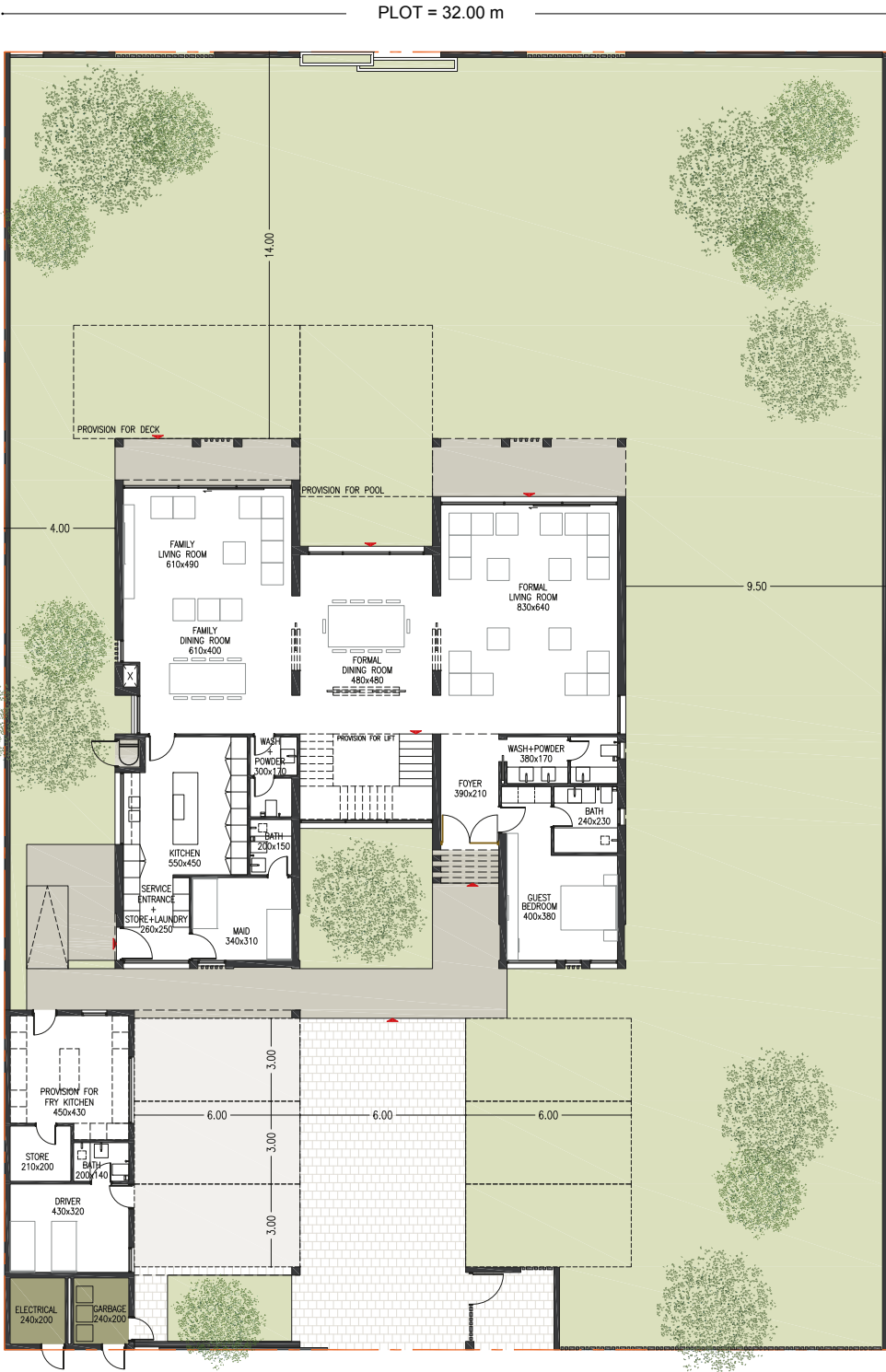
Ground Floor
